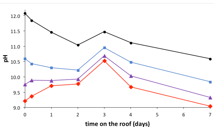
Figure 1. pH change of open unbuffered alkaline CN solution (1.0 L of 7.3 mM KCN (190 mg CN/L) with various initial pH values: \text{pH}_0 = 12.1 (black circles); \text{pH}_0 = 10.6 (blue squares); \text{pH}_0 = 9.75 (purple triangles); and \text{pH}_0 = 9.2 (red diamonds). Solutions were in unstirred open 2 L beakers exposed to sunlight on the building roof. Afternoon temperatures during the 7-day period were 32 – 34 °C, but on day 3 it reached 41 °C.
