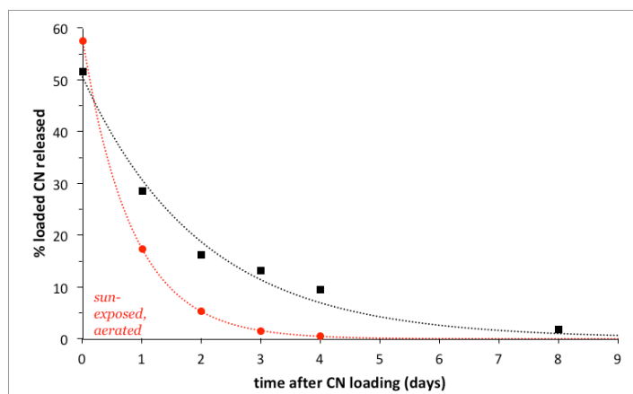
Figure 6. Kinetics of decline in acid-releasable CN from soil columns. Dark columns were wrapped with aluminum foil. Deaerated columns were flushed with N 2 (g). Data fit by non-linear regression to exponential decline: Black squares: dark, aerated columns, initial % = 50.5 ± 2.3 %, k = 0.50 \pm 0.04 \text{ dy}^{-1} ; R^2 = 0.985 ; red circles: sunlight-exposed, aerated columns, initial % = 57.60 ± 0.10 %, k = 1.198 \pm 0.005 \text{ dy}^{-1} ; R^2 = 0.999 .
